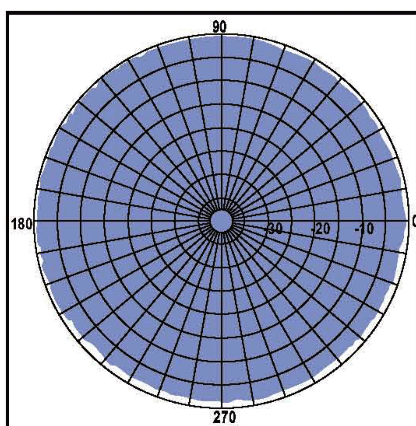
Horizontal pattern
