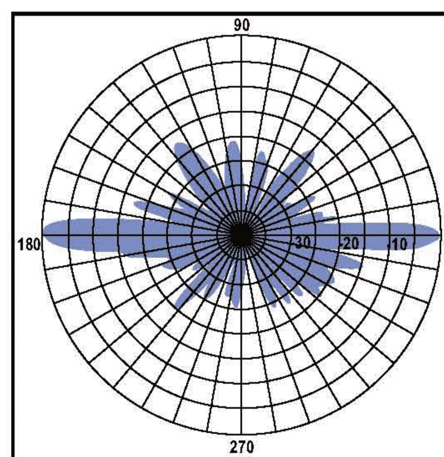
Vertical pattern
