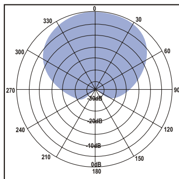
Horizontal pattern
