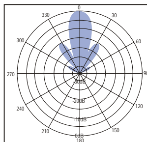
Vertical pattern
