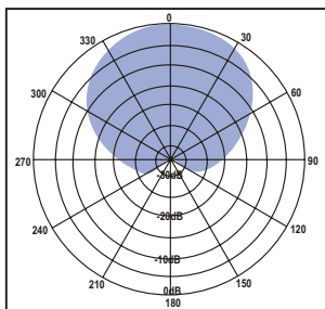
Horizontal pattern
