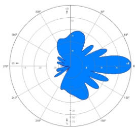
Vertical Pattern 824-896MHz
