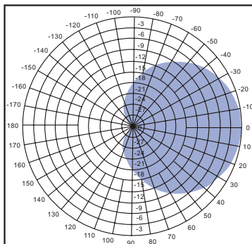
Vertical pattern 870-960 MHz
