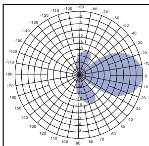
Vertical pattern 824-896 MHz
