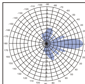
Vertical pattern 1850-1990 MHz
