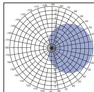
Vertical pattern 1850-1990 MHz
