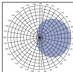
Vertical pattern 824-896 MHz
