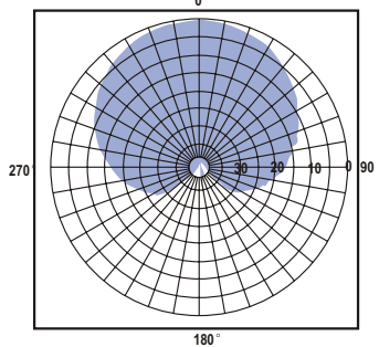
Horizontal pattern
