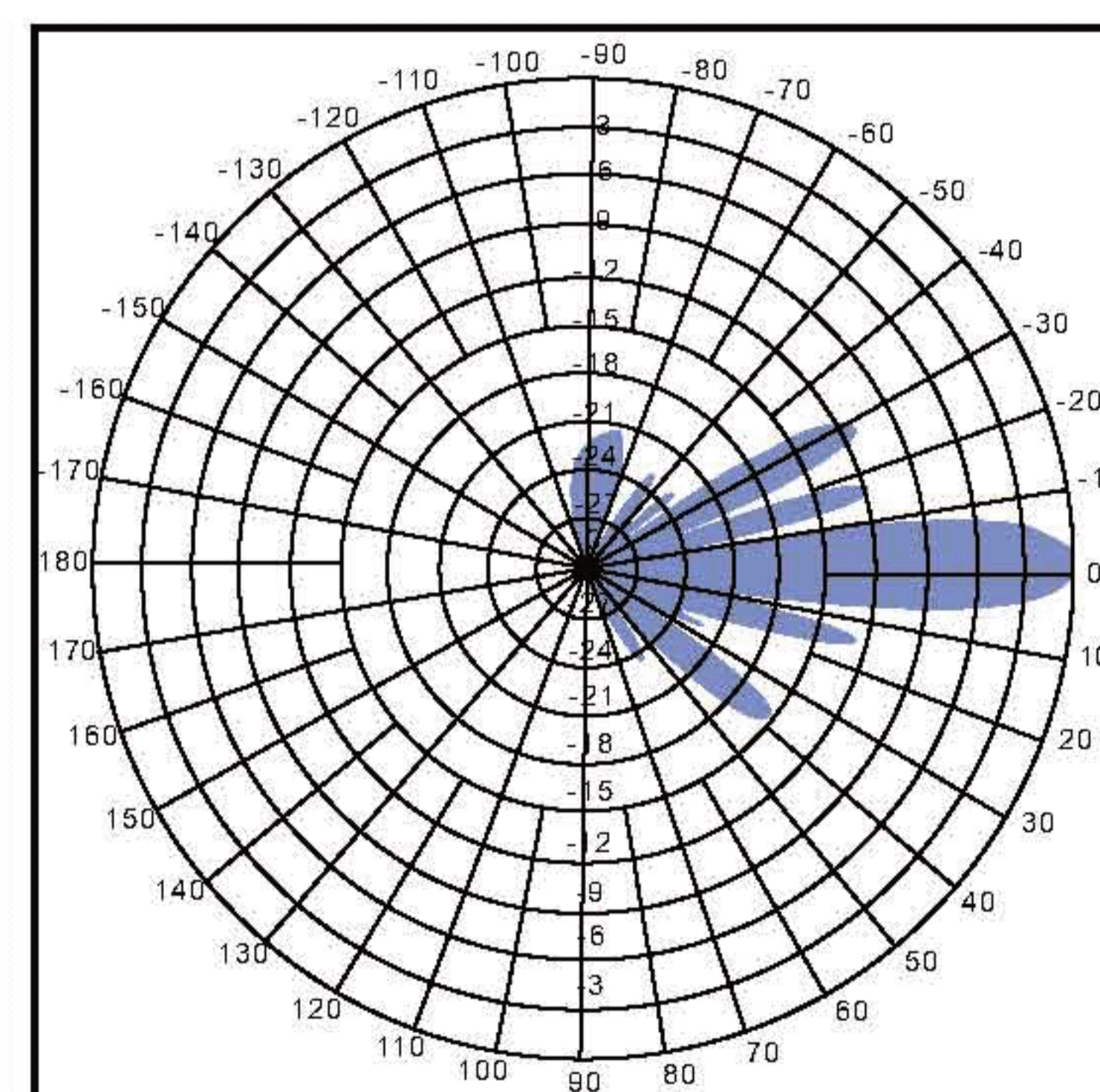
Vertical pattern
