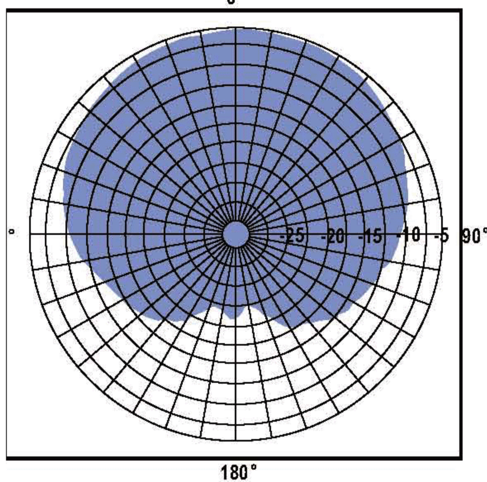
Horizontal pattern 0°
