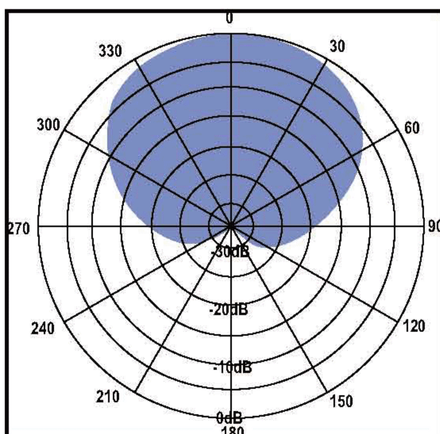
Horizontal pattern
