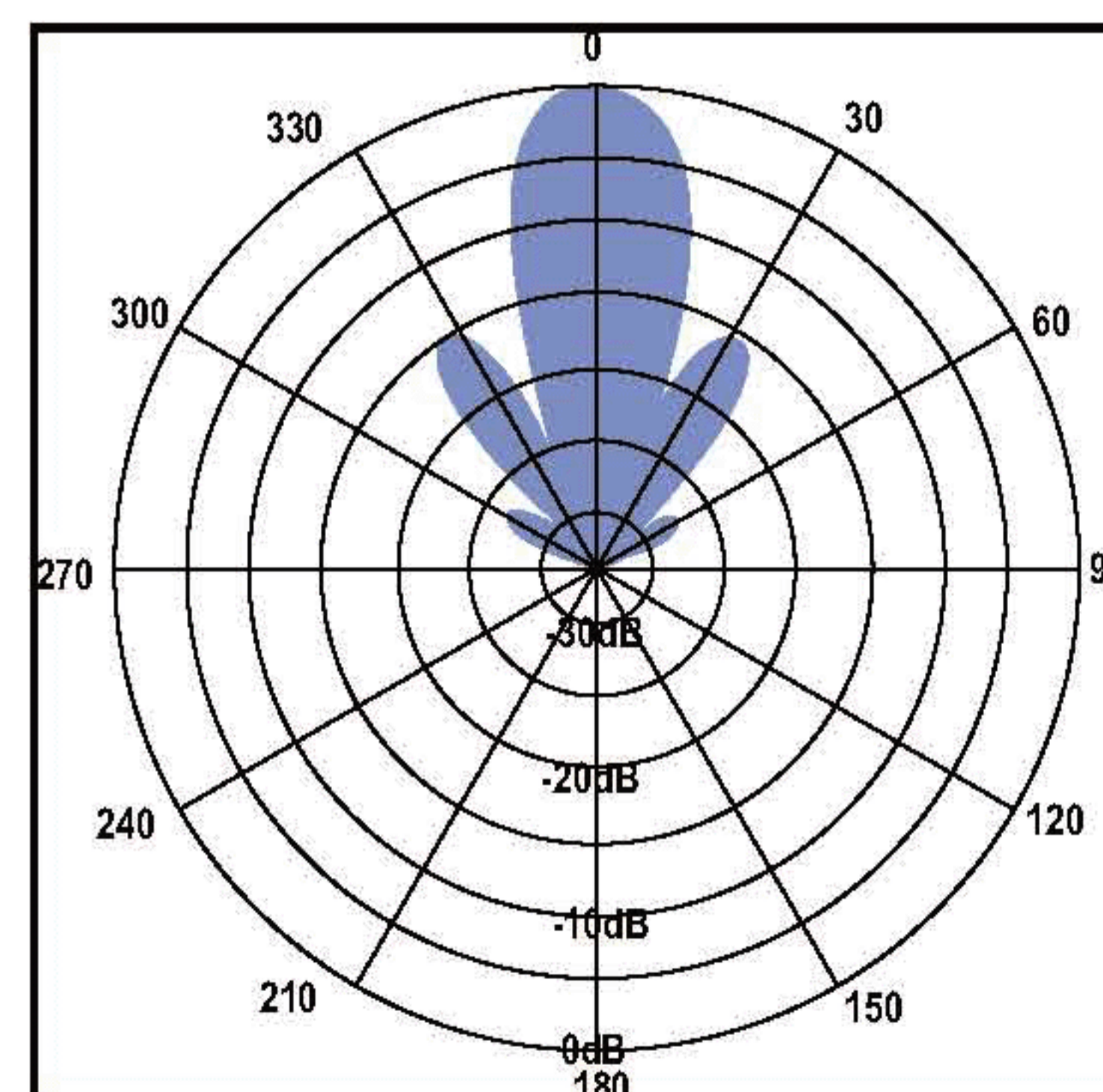
Vertical pattern
