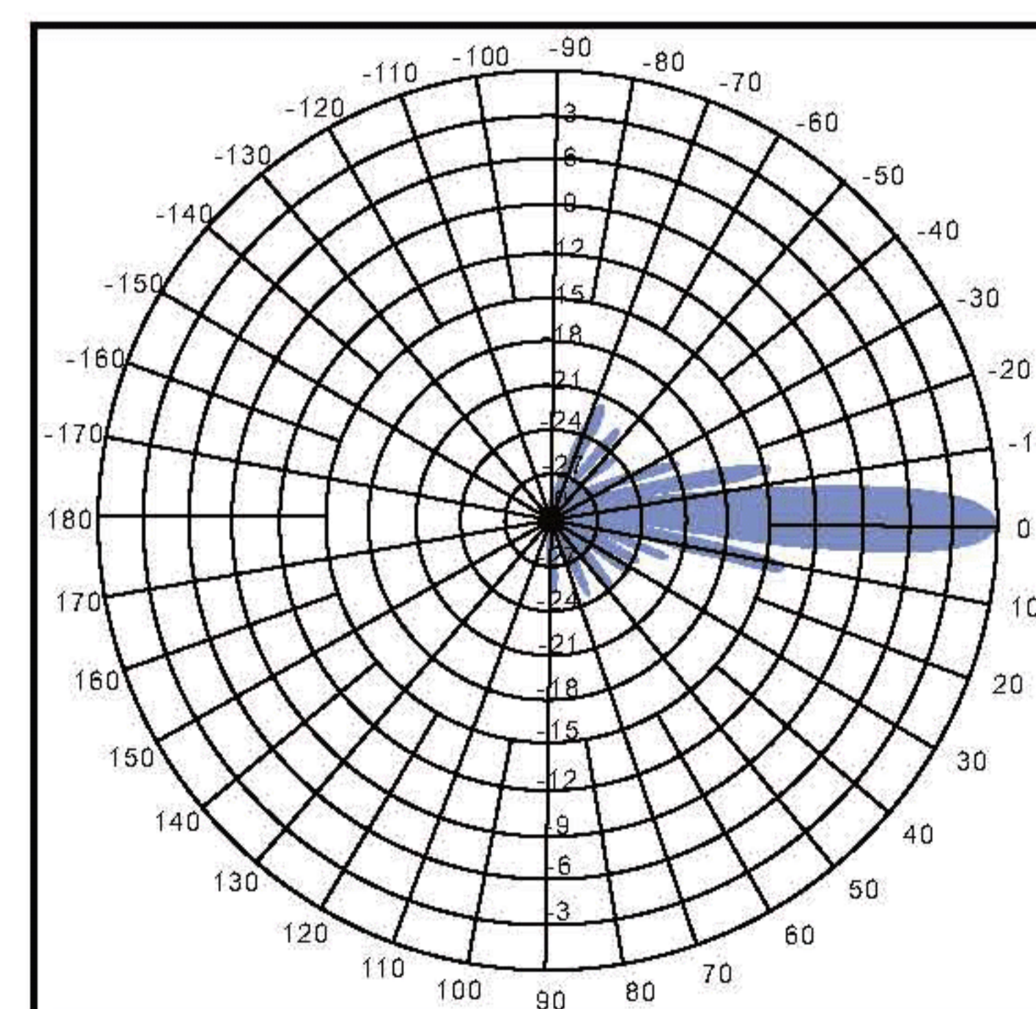
Vertical pattern
