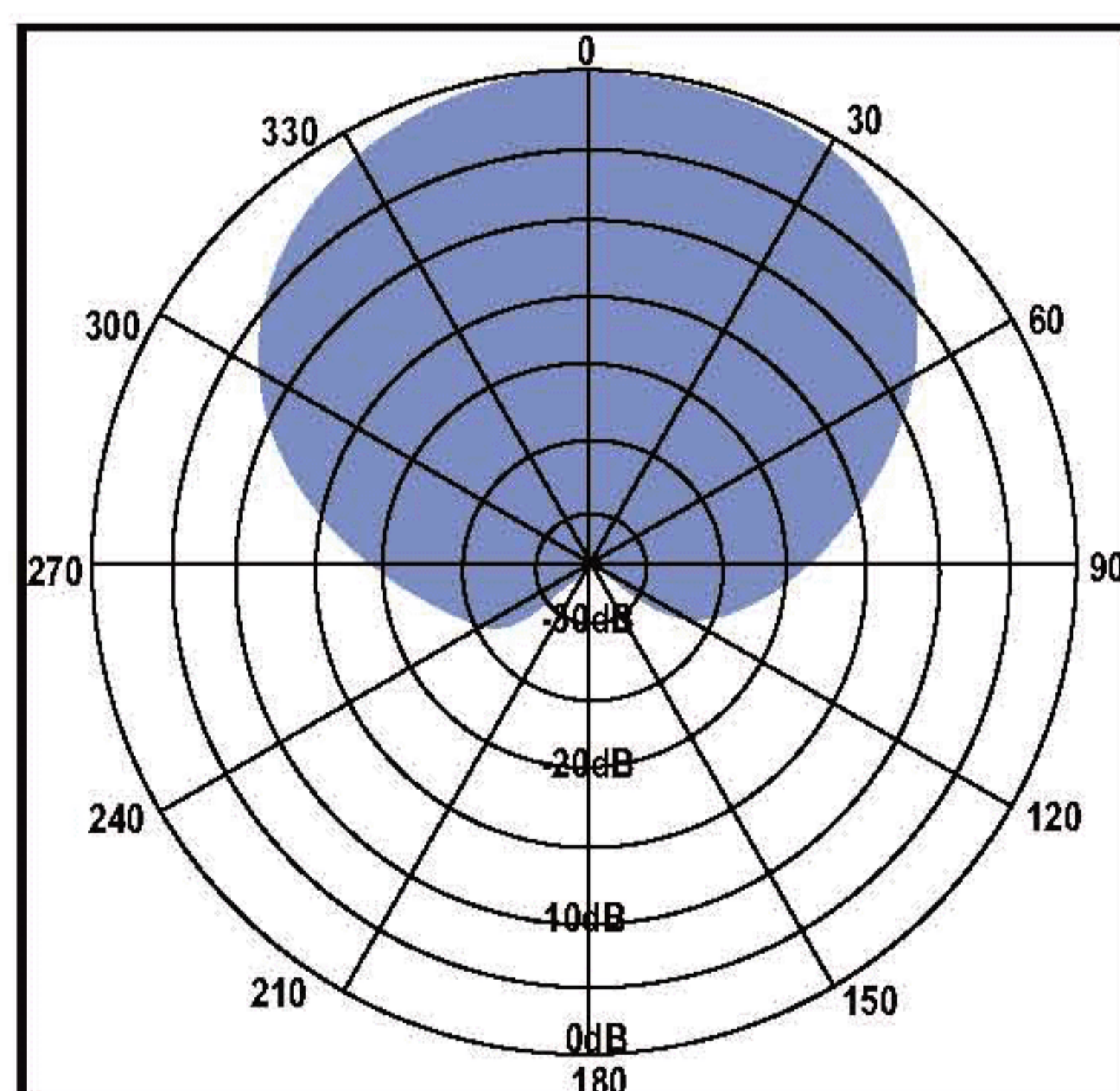
Horizontal pattern
