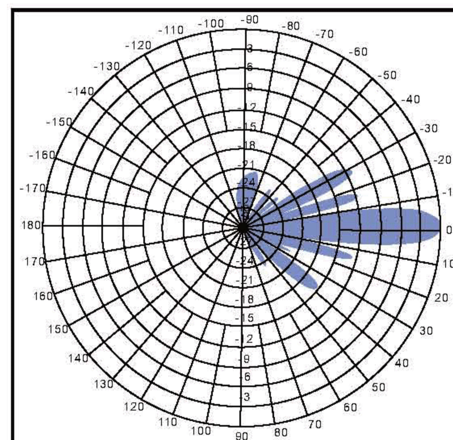
Vertical pattern
