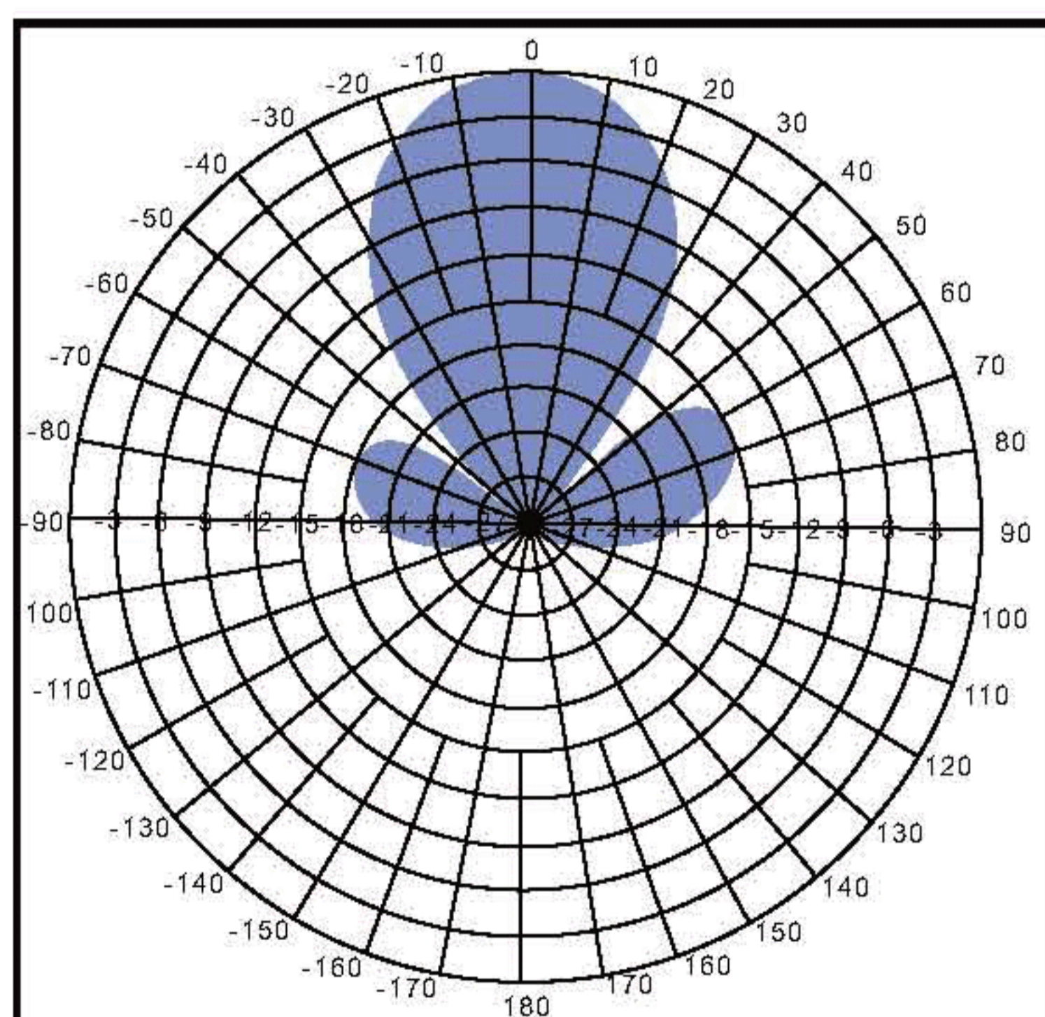
Horizontal pattern
